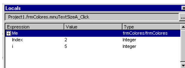
Figura 2.15. Ventana Locals .
